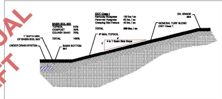
TYP. SIDE SLOPE SECTION
