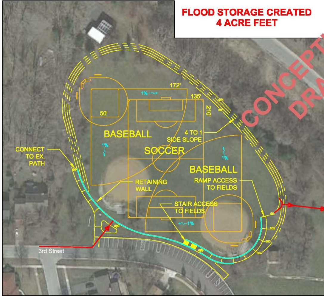
EAST END PARK SITE DEVELOPMENT PLAN
