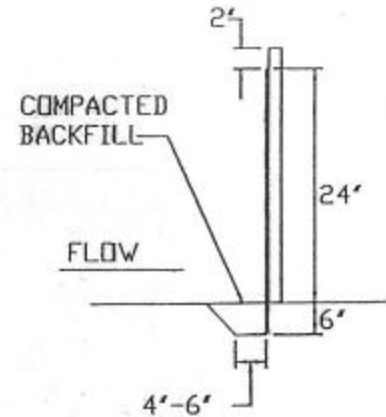
SILT FENCE DETAIL
